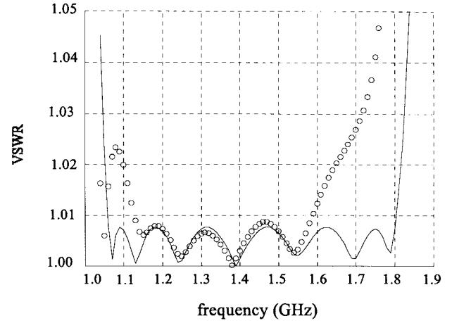
Fig. 21. The optimal ideal analytical model response (—) and the response of the nonideal analytical model (o) at the starting point for the seven-section waveguide transformer.
