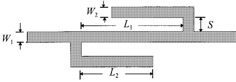
Fig. 2. The DFS filter [5].
