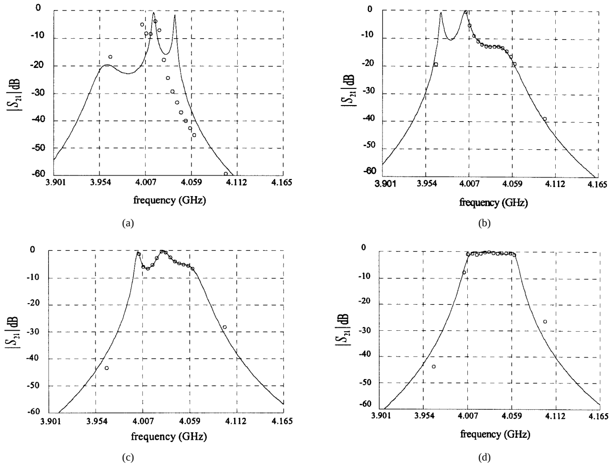
Fig. 9. The coarse-model response (—) at the extracted point and the fine-model response (o) corresponding to the second, third, fourth, and fifth iterations.
